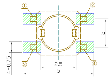
P.C.B MOUNTING PATTERN DIMENSION the following soldering are recommended for reflow soldering
